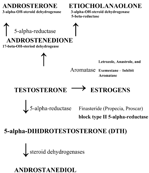
Figure 3 Testosterone metabolism.
